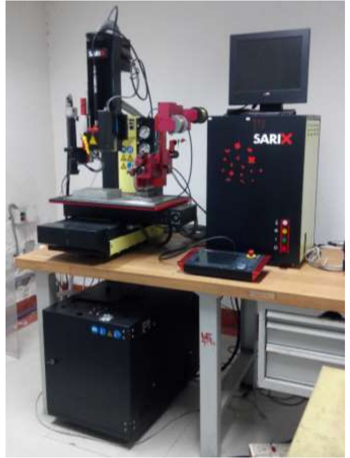
Micro EDM
