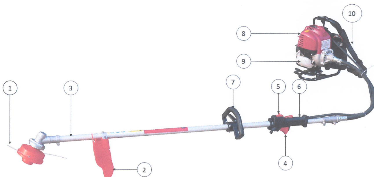
FIG. 1: SCHEMATIC VIEW OF BRUSH CUTTER
