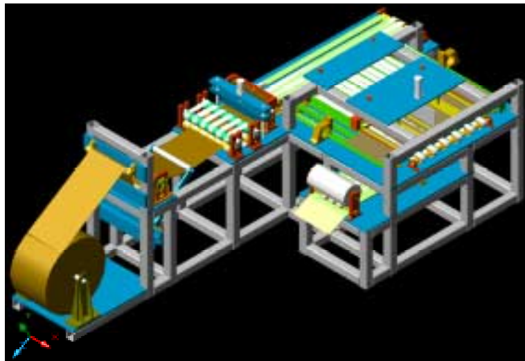
3D View of automatic jute bag making machine
